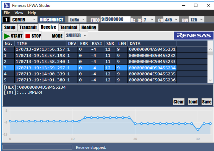
Reception mode (Sniffer)
