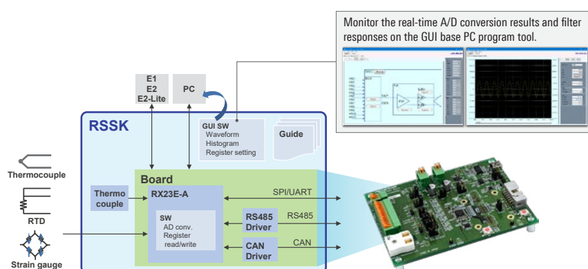
Renesas Solution Starter Kit for RX23E-A
