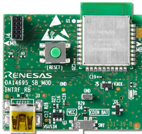
Figure 1. DA14695 BTLE Development Kit DB
