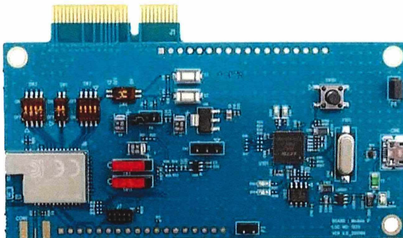
Figure 1. DA16200MOD-DEVKT Ultra-Low Power Wi-Fi Modules Development Kit
