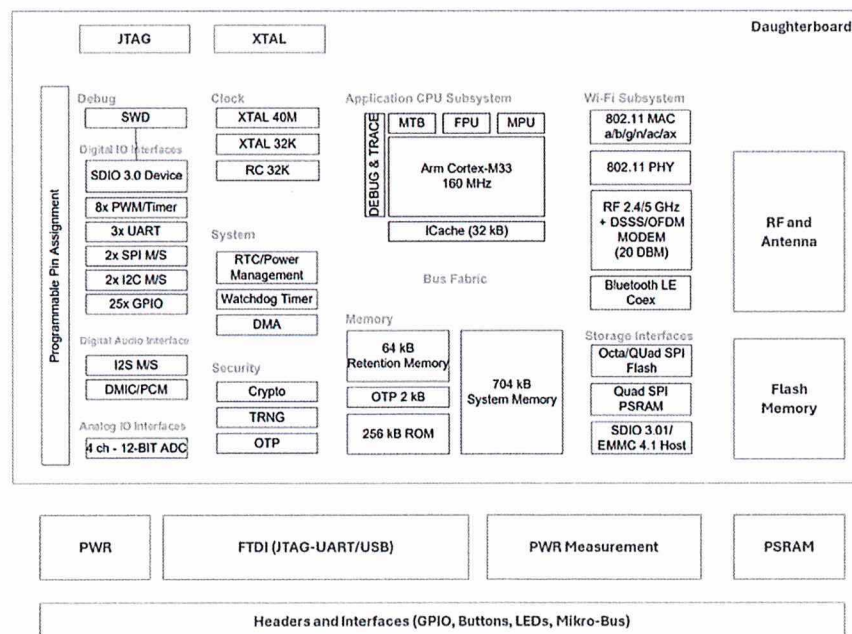
Figure 1. RA6W1 Development Kit
