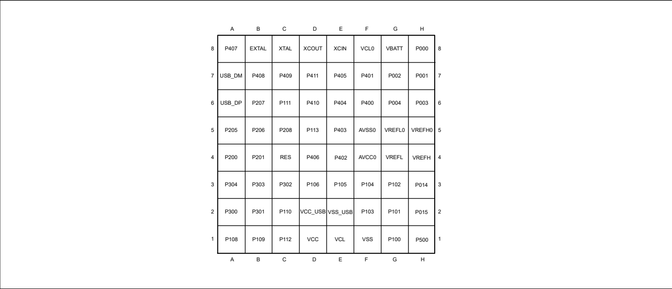
Figure 1.6 Pin assignment for BGA 64-pin (top view, pad side down)
