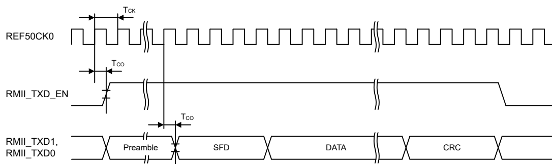
Figure 2.50 RMII transmission timing
