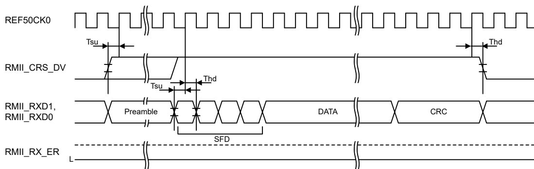
Figure 2.51 RMII reception timing in normal operation
