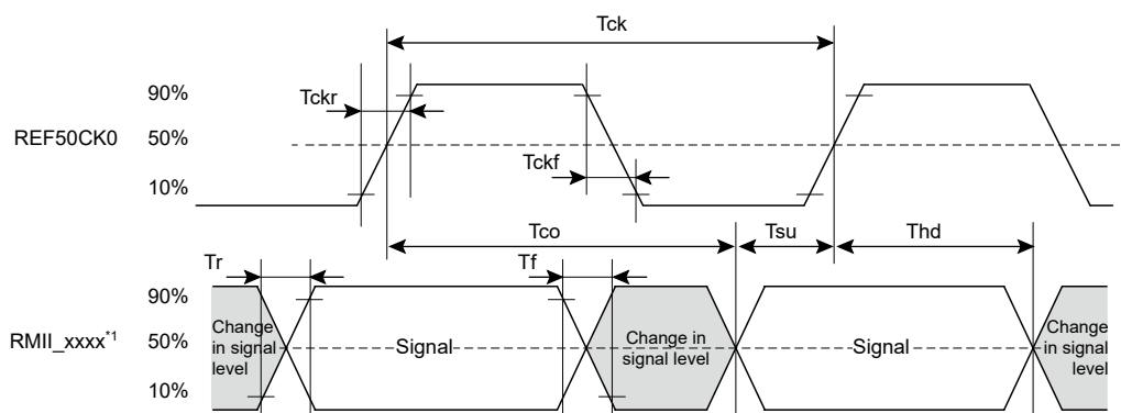
Figure 2.49 REF50CK0 and RMII signal timing
