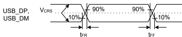
Figure 2.56 USB_DP and USB_DM output timing in full-speed mode
