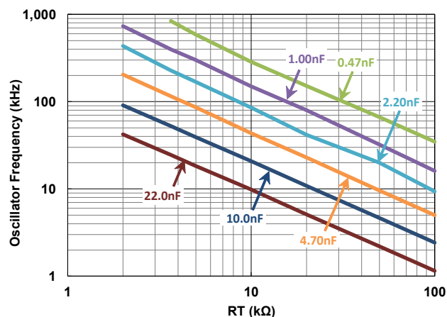
Figure 4. Oscillator Frequency vs RT and CT (+125°C)
