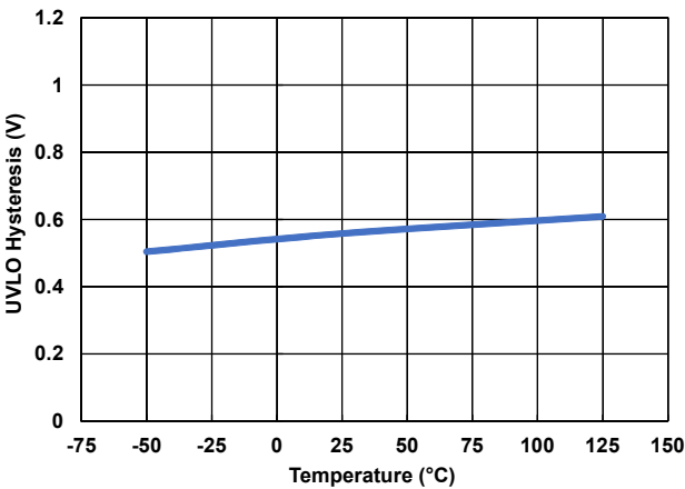
Figure 52. V_{HYS} vs Temperature
