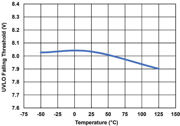
Figure 51. V_{STOP} vs Temperature
