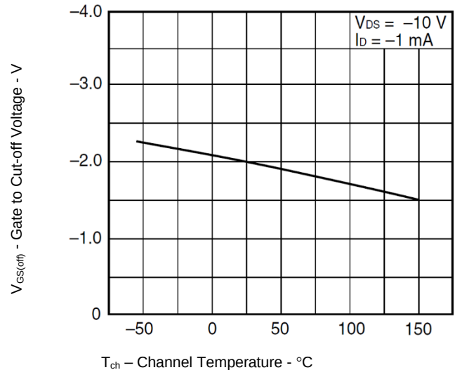
GATE CUT-OFF VOLTAGE vs. CHANNEL TEMPERATURE
