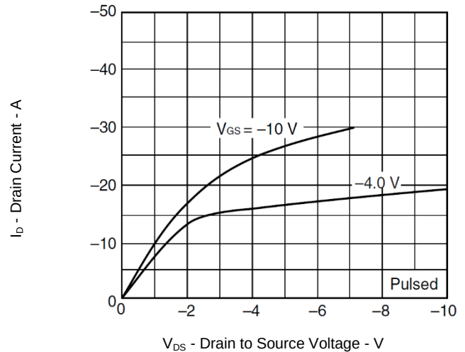
DRAIN CURRENT vs. DRAIN TO SOURCE VOLTAGE
