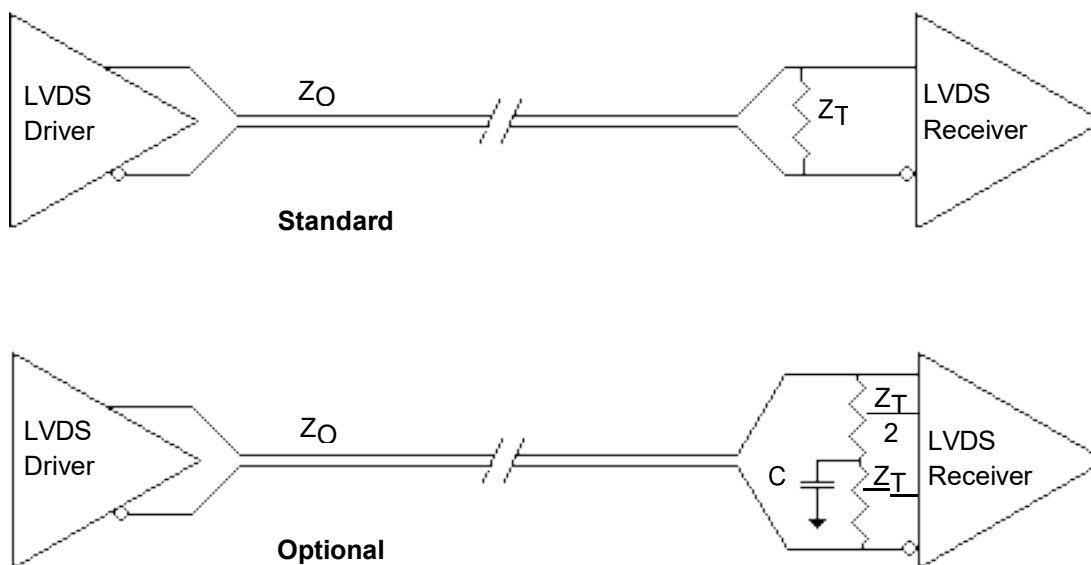
Figure 11. Standard and Optional Terminations
