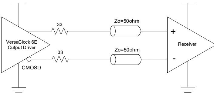
Figure 19. LVCMOS Termination
