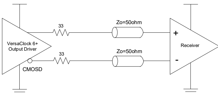
Figure 19. LVCMOS Termination
