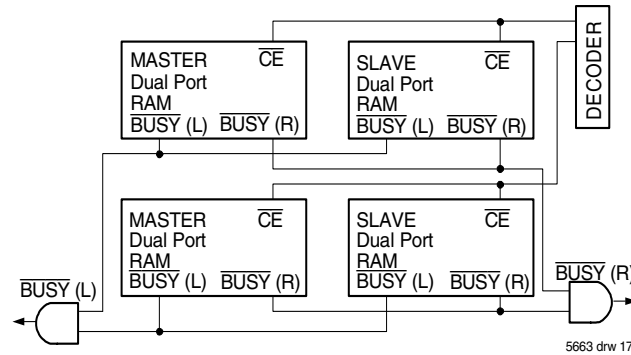
Figure 3. Busy and chip enable routing for both width and depth expansion with IDT70T16/5 RAMs.
