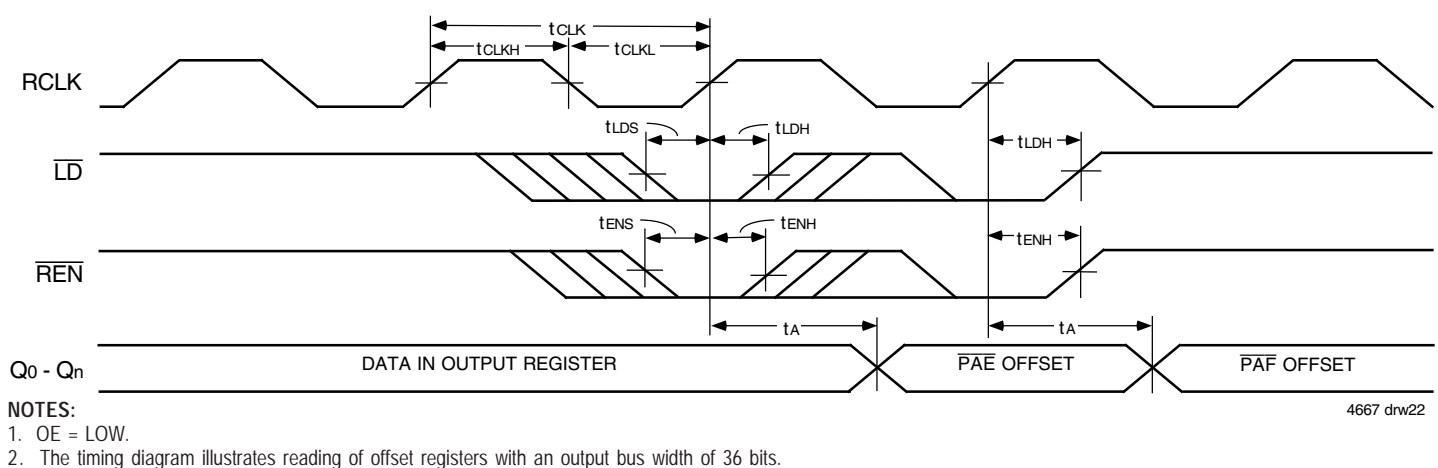
Figure 17. Parallel Read of Programmable Flag Registers (IDT Standard and FWFT Modes)
