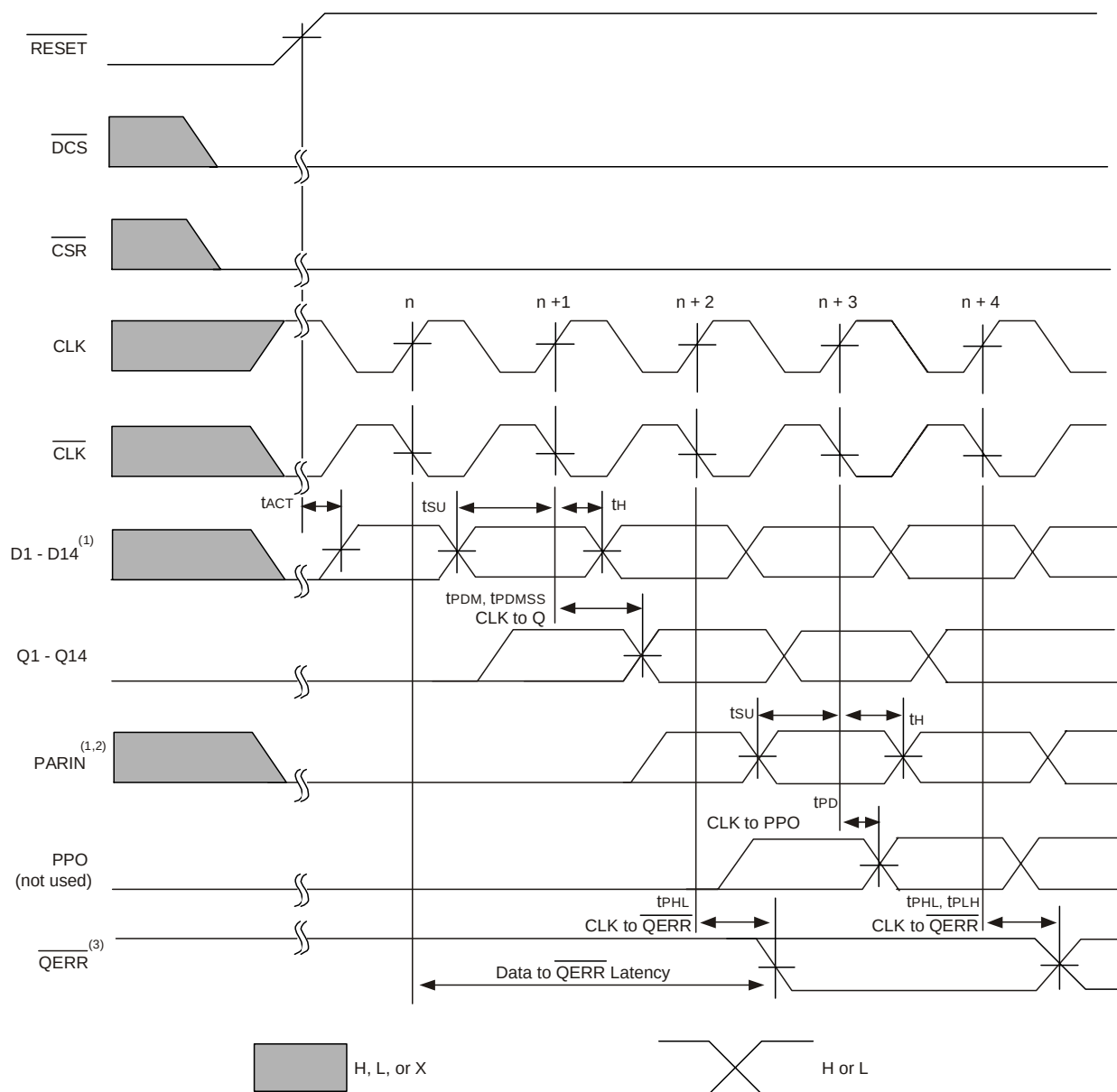
Timing Diagram for the Second SSTUBF32866B (1:2 Register-B Configuration) Device Used in a Pair; C0 = 1, C1 = 1, \overline{\text{RESET}} Switches from L to H
