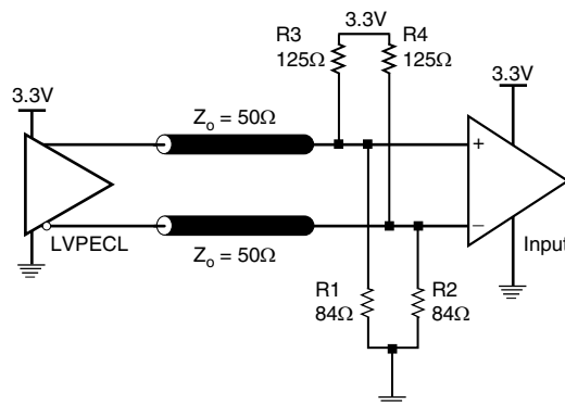
Figure 22. 3.3V LVPECL Output Termination
