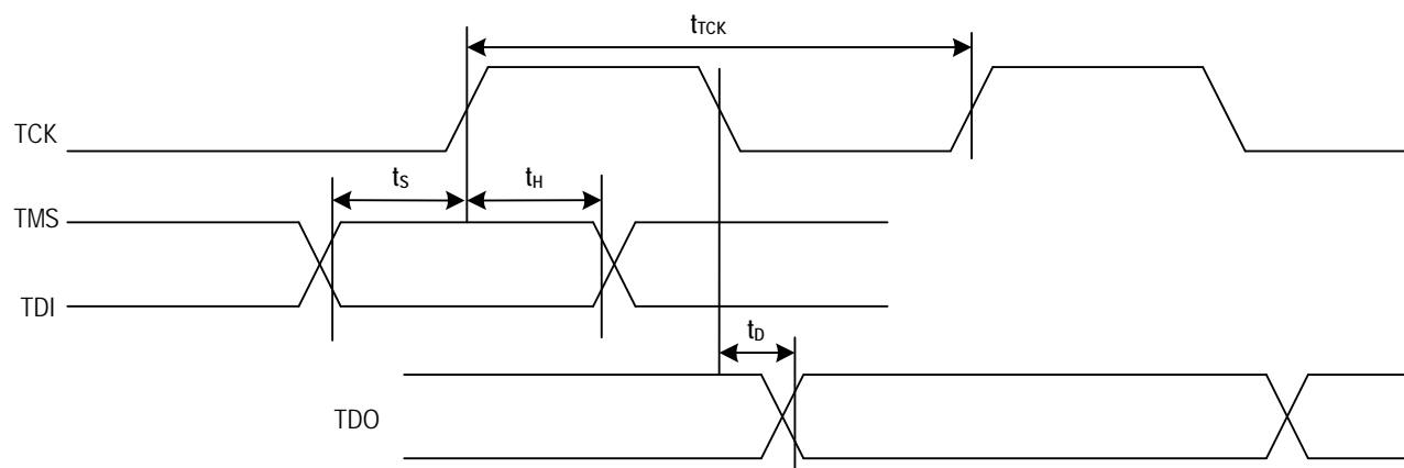
Figure 20. JTAG Interface Timing Diagram
