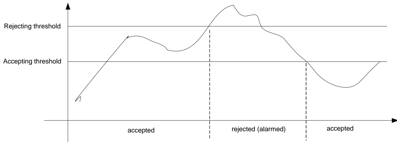
Figure 8. Hysteresis Frequency Monitoring
