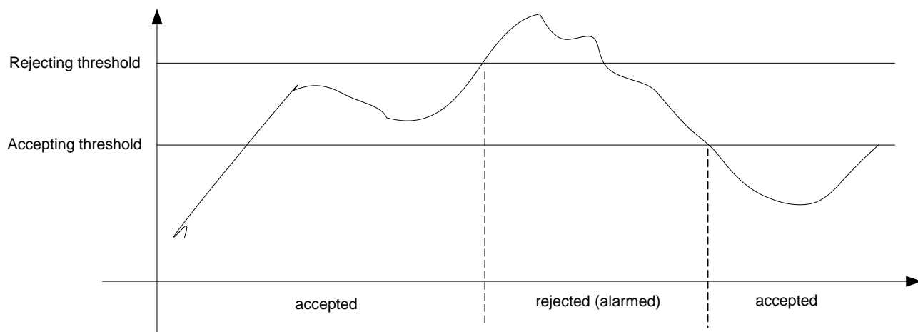
Figure 8. Hysteresis Frequency Monitoring
