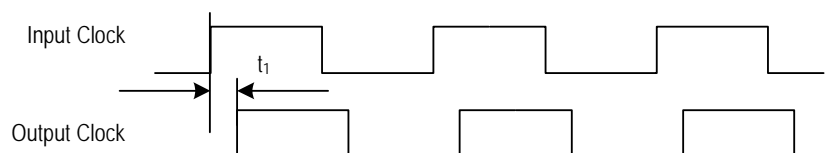
Figure 25. Input / output clock timing
