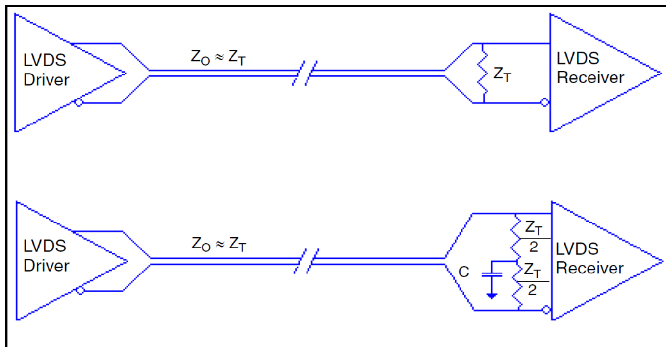
Figure 23. Recommended LVDS Output Port Line Termination
