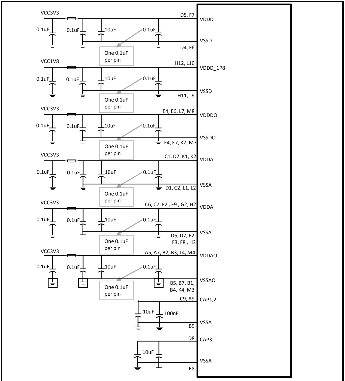
Figure 12. 82P33741 Power Decoupling Scheme
