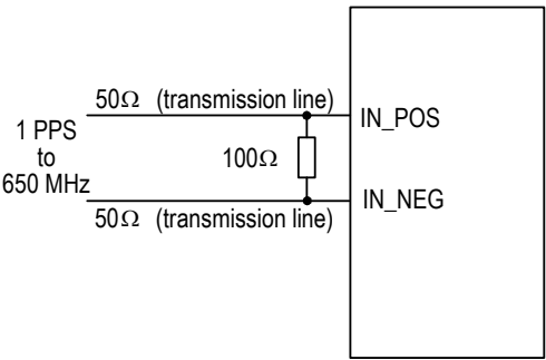
Figure 38. Recommended LVDS Input Port Line Termination
