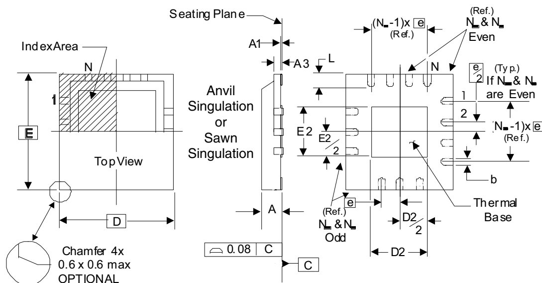
Package Outline - K Suffix for 32 Lead VFQFN
