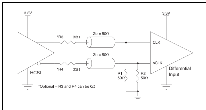
Figure 2D. CLK/nCLK Input Driven by a 3.3V HCSL Driver
