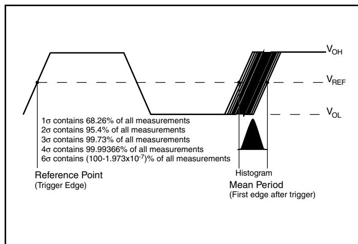
Period Jitter
