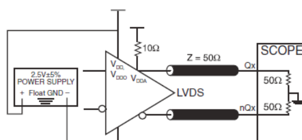
2.5V CORE/2.5V OUTPUT LOAD AC TEST CIRCUIT
