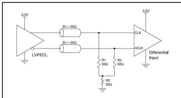
Figure 2B. CLK/ \overline{\text{CLK}} Input Driven by a 3.3V LVPECL Driver
