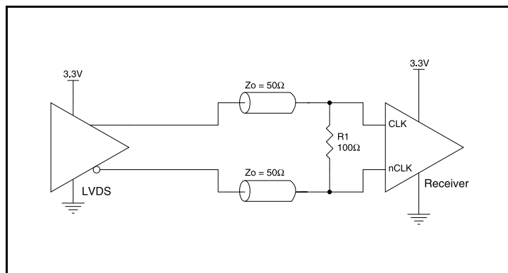
Figure 2D. CLK/ \overline{\text{CLK}} Input Driven by a 3.3V LVDS Driver
