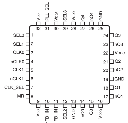
ICS8745BI 32-Lead LQFP 7mm x 7mm x 1.4mm package body Top View
