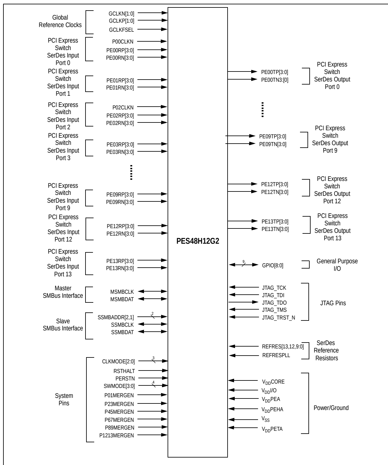
Figure 4 PES48H12G2 Logic Diagram
