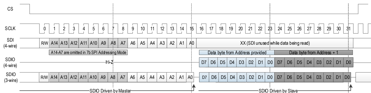
Figure 20. SPI Sequencing
