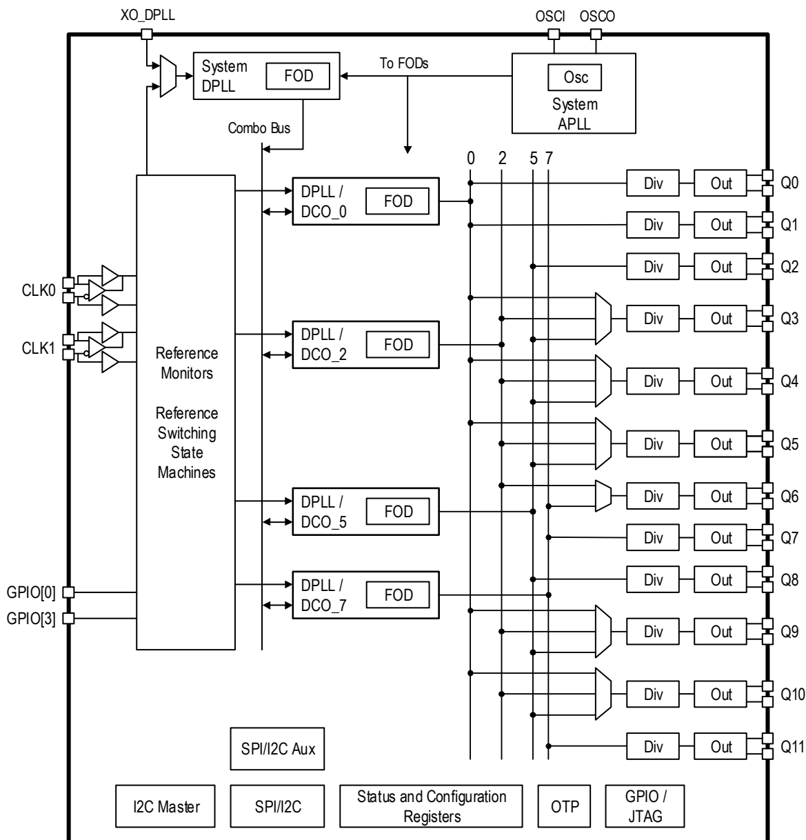
Figure 1. Block Diagram
