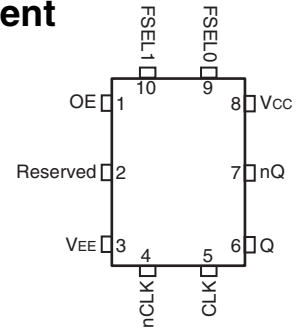
ICS8N3PGDAMBKI-025
