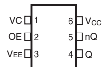
IDT8N3SV75 6-lead ceramic 5mm x 7mm x 1.55mm package body CD Package Top View
