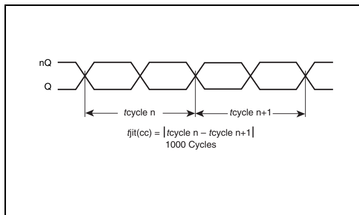
Cycle-to-Cycle Jitter
