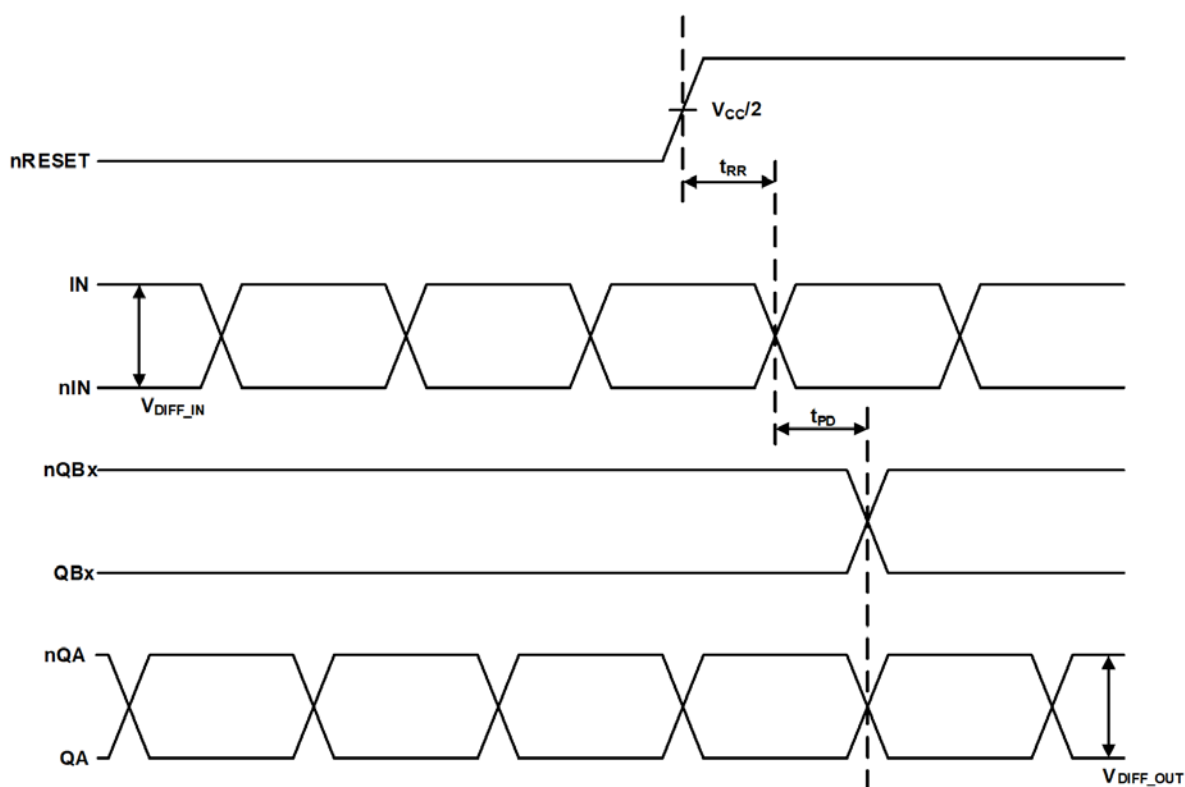
Figure 1. nRESET Timing Diagram
