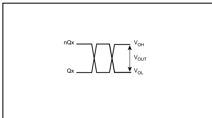
LVDS Output Voltage Level
