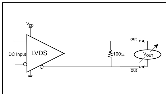
LVDS Output Voltage Swing
