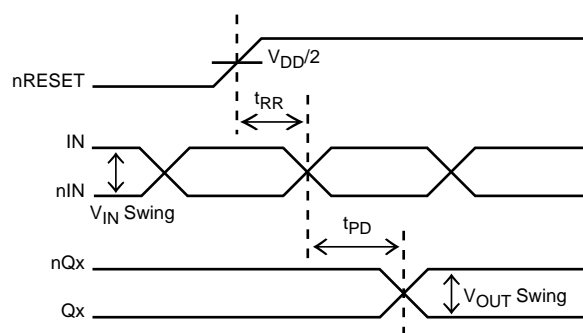
Figure 1. nRESET Timing Diagram
