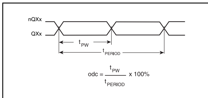
Differential Output Duty Cycle/Output Pulse Width/Period
