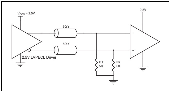
Figure 8C. 2.5V LVPECL Driver Termination Example
