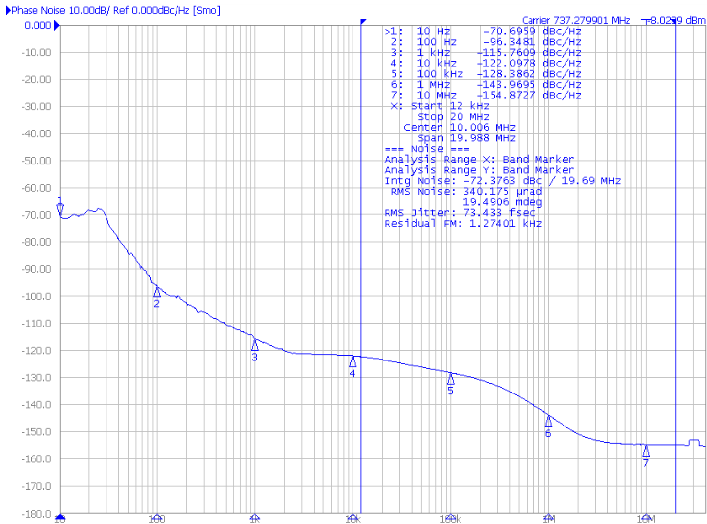
Figure 11. 737.28MHz Output Phase Noise ( f_{VCXO} = 30.72\text{MHz} )
