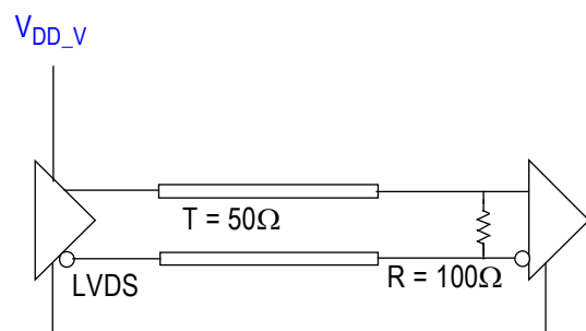
Figure 12. LVDS (STYLE = 0) Output Termination
