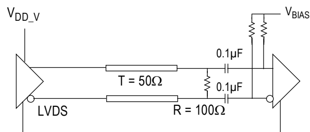
Figure 13. LVDS (STYLE = 0) AC Output Termination
