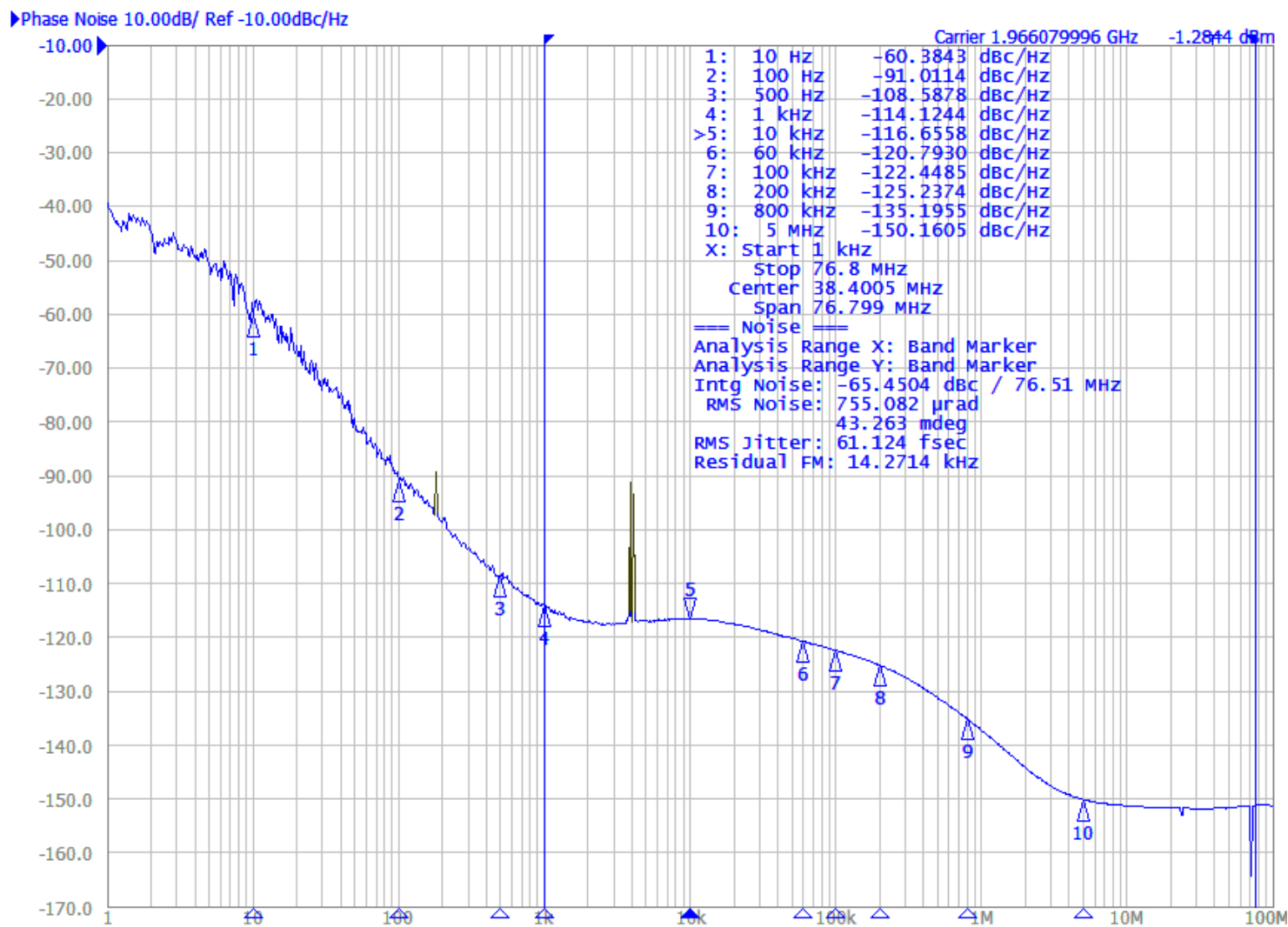
Figure 9. 1966.08MHz Output Phase Noise
