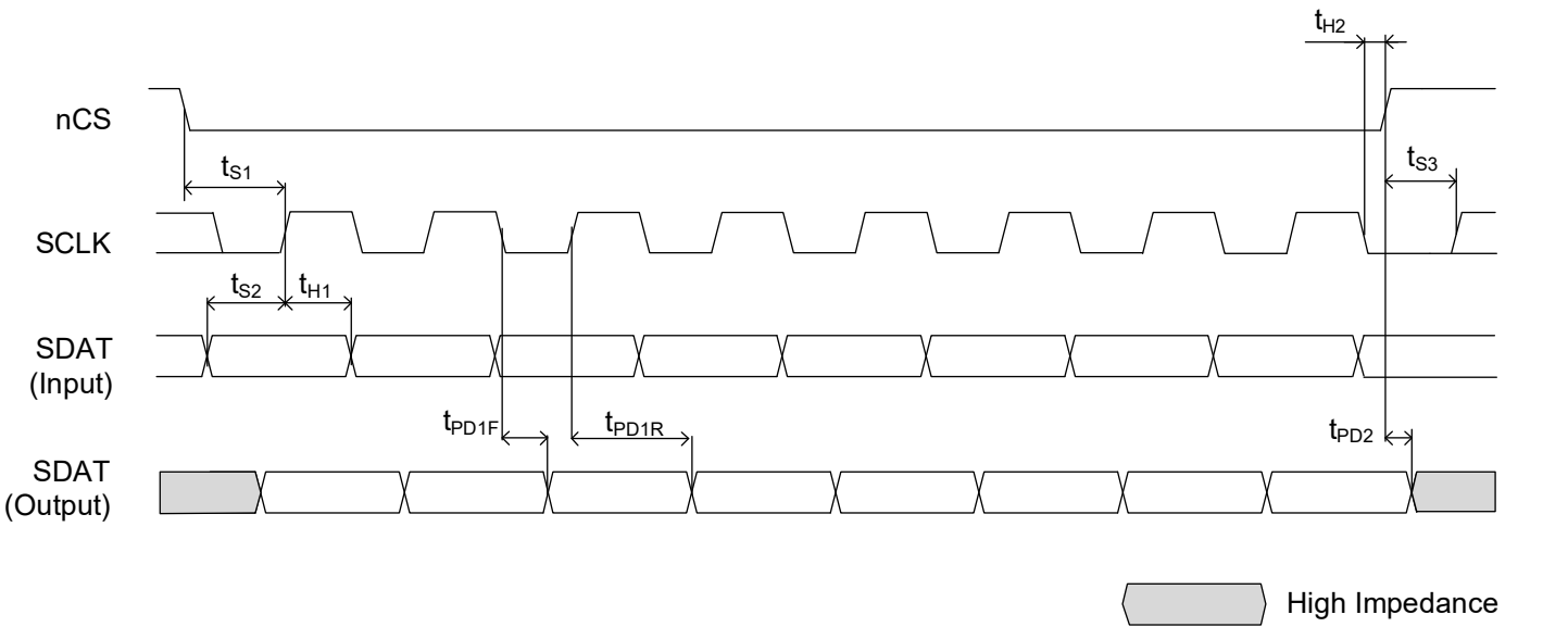
Figure 7. SPI Timing Diagram
