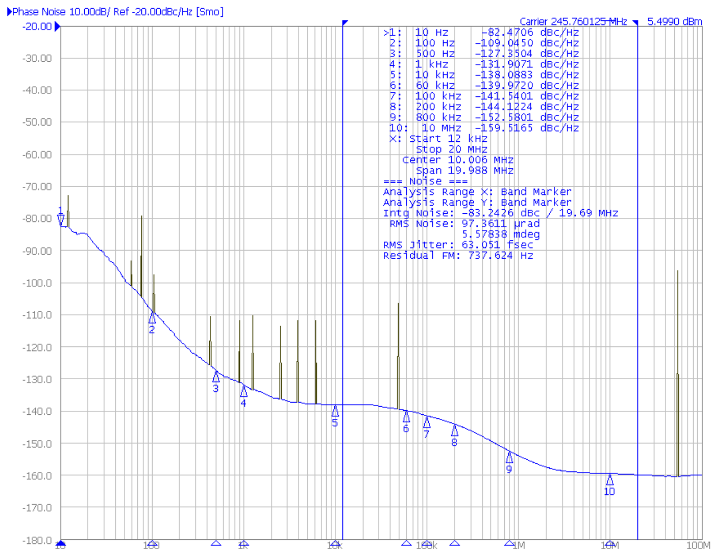
Figure 11. 245.76MHz Output Phase Noise
