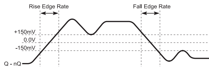
Figure 8. Differential Measurement Points for Rise/Fall Time Edge Rate
