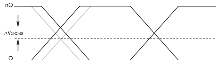
Figure 9. Single-ended Measurement Points for Delta Cross Point
