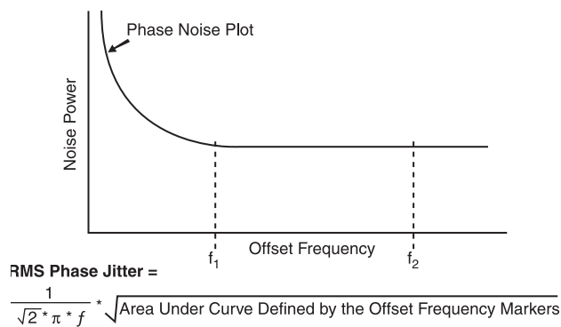
Figure 6. RMS Phase Jitter
