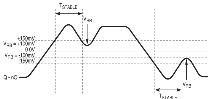
Figure 13. Differential Measurement Points for Duty Cycle/Period
