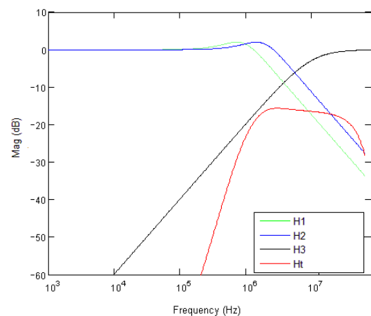
Figure 29. PCIe Gen 3 Magnitude of Transfer Function
