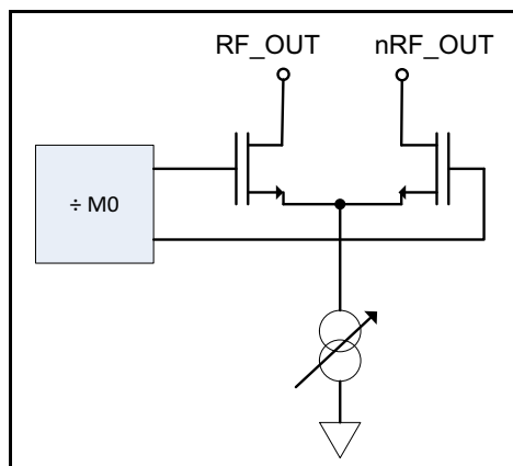
Figure 4. Output Stage
