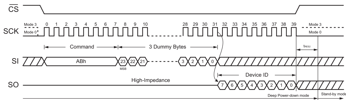
Figure 20. Release Power-Down / Device ID Command
