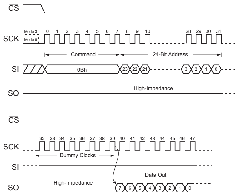
Figure 11. Fast Read Command
