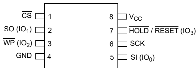
Figure 1. AT25EU0011A Pin Assignments, 8-pin SOIC 150-mil (Top View)
