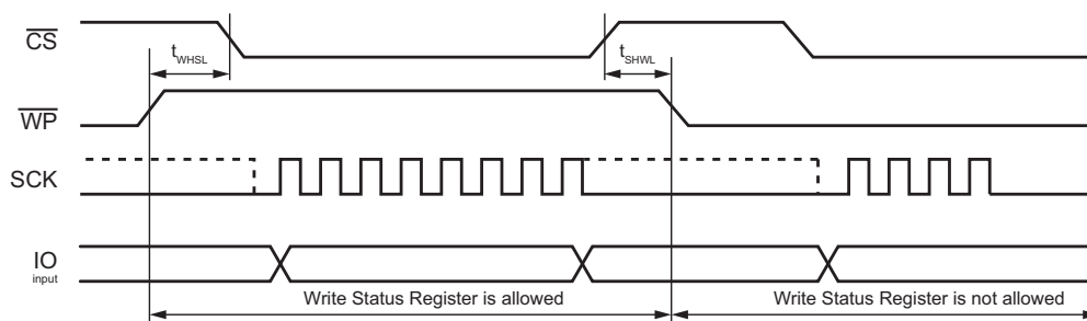
Figure 47. \overline{\text{WP}} Timing
