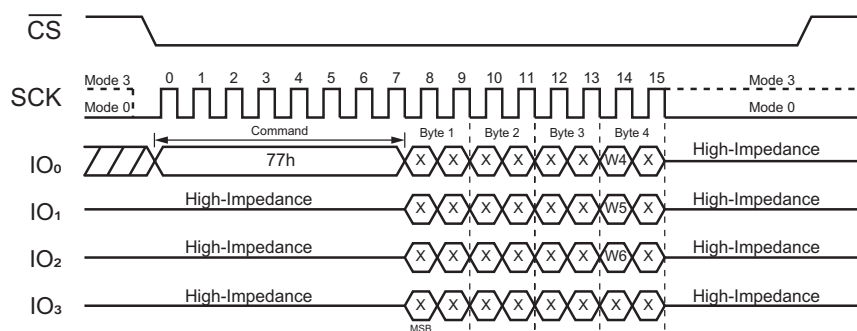
Figure 18. Set Burst with Wrap Command
