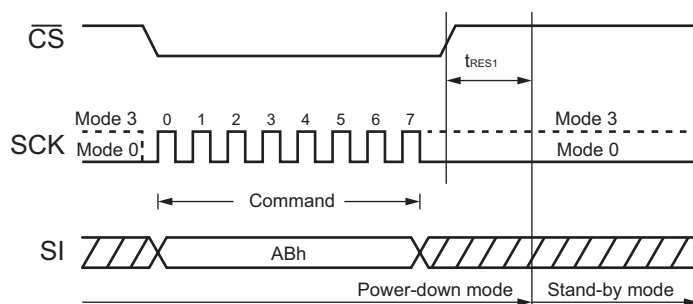
Figure 19. Release Power-Down Command
