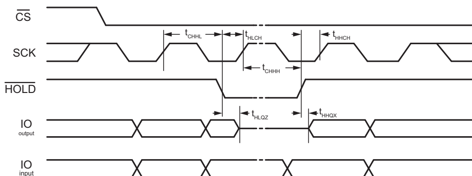
Figure 46. HOLD Timing
