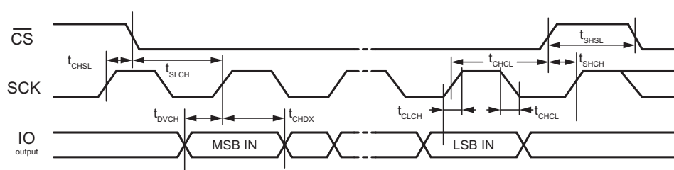
Figure 45. Serial Input Timing
