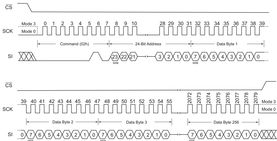
Figure 27. Page Program Command
