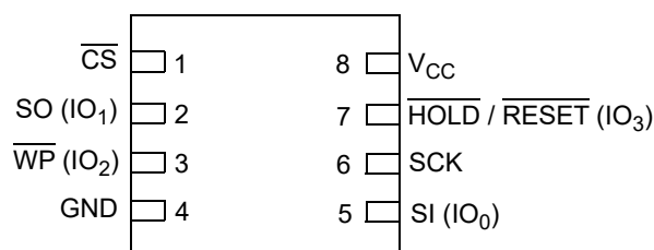
Figure 2. AT25EU0011A Pad Assignments, 8-pad DFN 2x3 mm (Top View)
