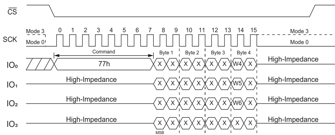
Figure 18. Set Burst with Wrap Command
