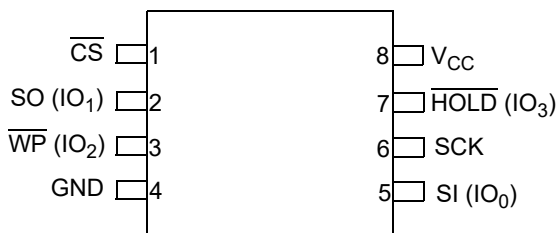
Figure 1. AT25EU0041A Pin Assignments, 8-pin SOIC 150-mil (Top View)
