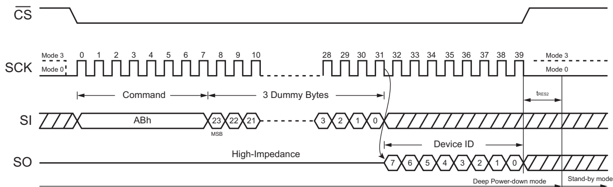
Figure 20. Release Power-Down / Device ID Command
