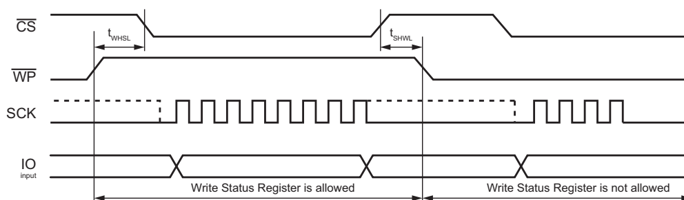
Figure 47. WP Timing
