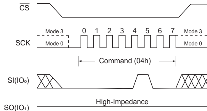
Figure 6. Write Disable Command, SPI Mode
