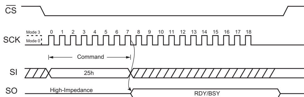
Figure 8. Active Status Interrupt Command
