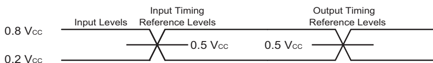
Figure 43. AC Measurement I/O Waveform
