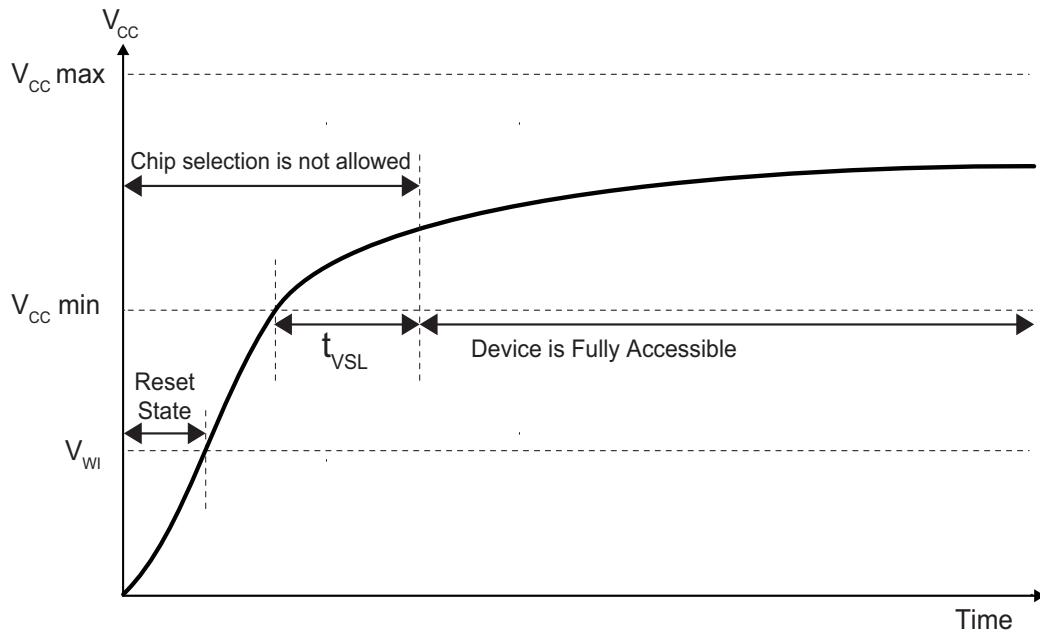
Figure 42. Power-Up Timing and Voltage Levels
