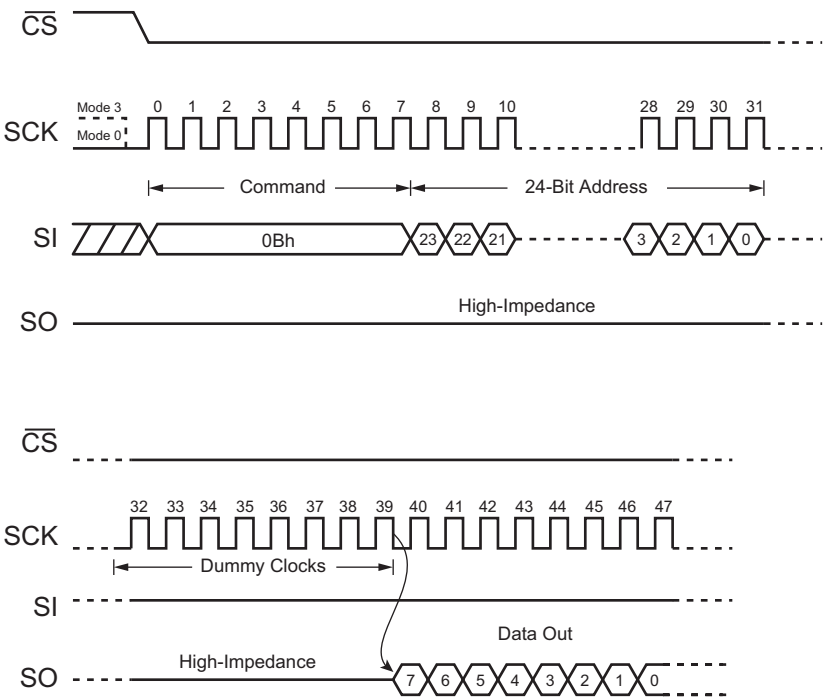
Figure 11. Fast Read Command
