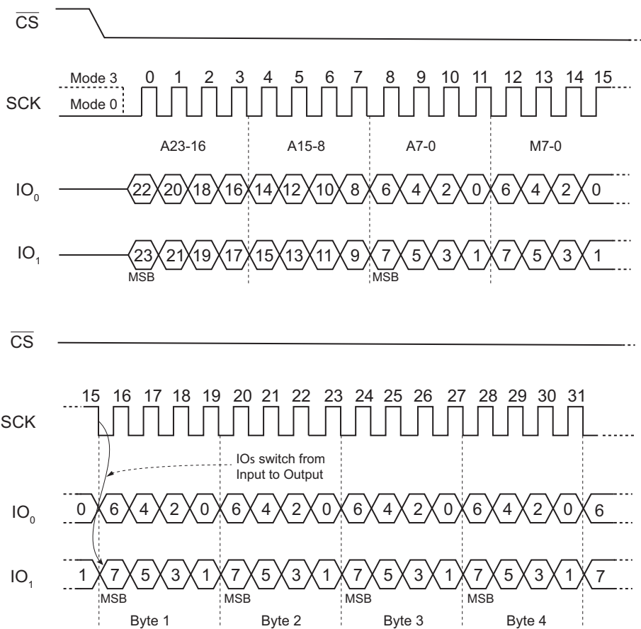
Figure 14. Fast Read Dual I/O Command (Previous command M5-4=10)
