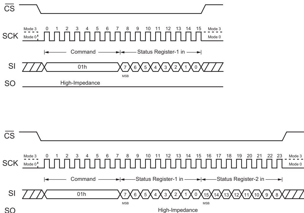
Figure 9. Write Status Register Command
