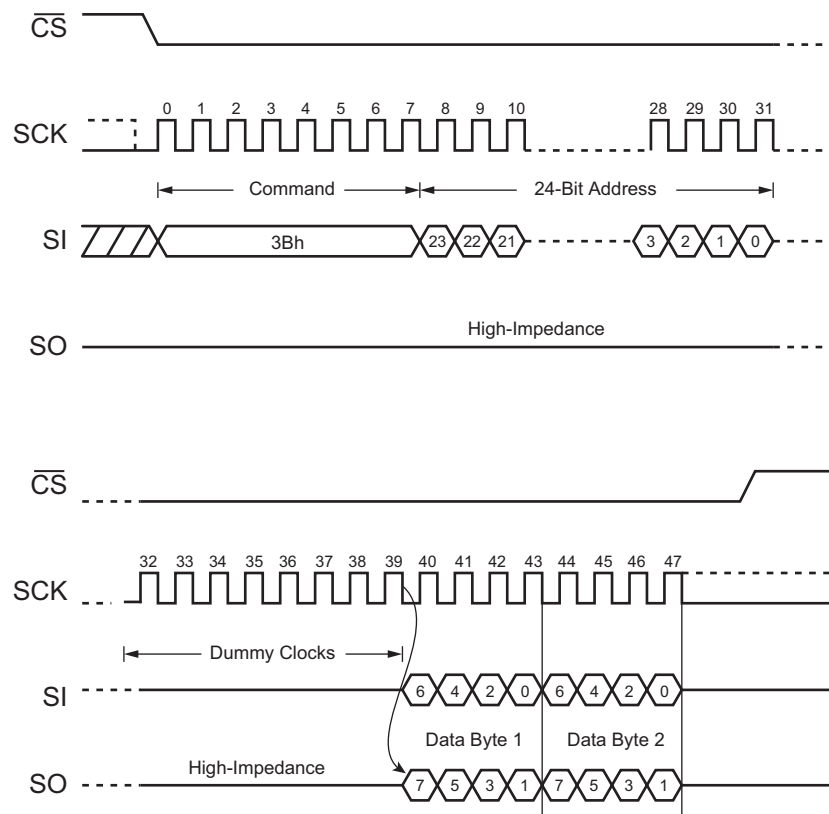
Figure 12. Fast Read Dual Output Command
