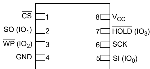
Figure 2. AT25EU0041A Pad Assignments, 8-pad DFN 2x3 mm (Top View)
