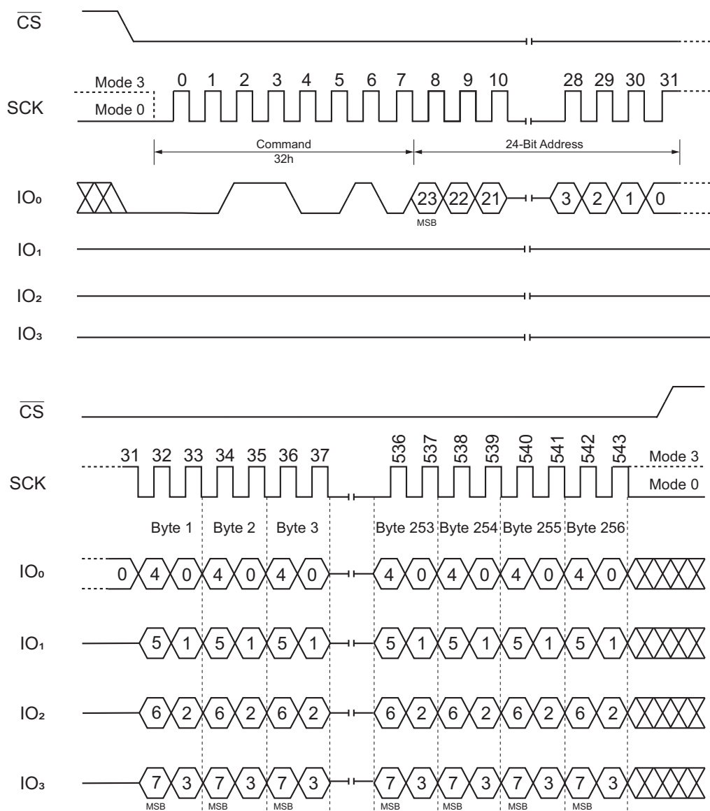
Figure 29. Quad Input Page Program Command
