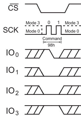
Figure 153. Global Block Unlock (QPI Mode)
