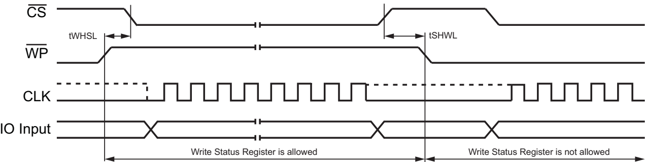
Figure 160. \overline{\text{WP}} Timing
