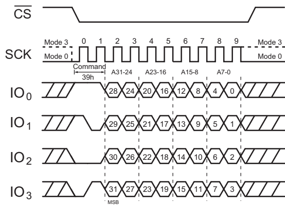
Figure 149. Individual Block Unlock (QPI Mode, Four-Byte Address Mode)
