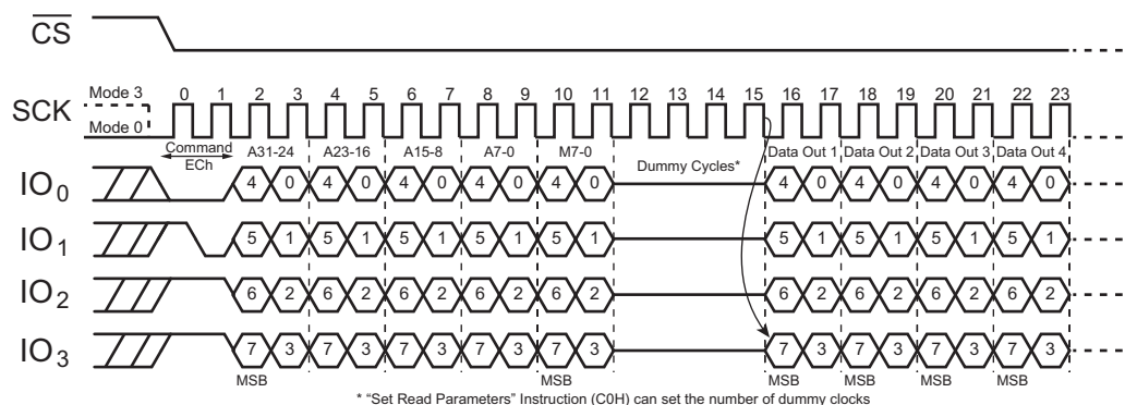
Figure 61. Fast Read Quad I/O with Four-Byte Address (QPI Mode; Initial command or previous M5-4≠10)
