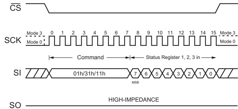
Figure 13. Write Status Register Sequence Diagram 01h, 31h, 11h One-Byte (SPI Mode)
