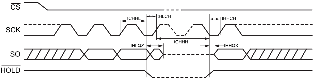
Figure 159. \overline{\text{HOLD}} Timing
