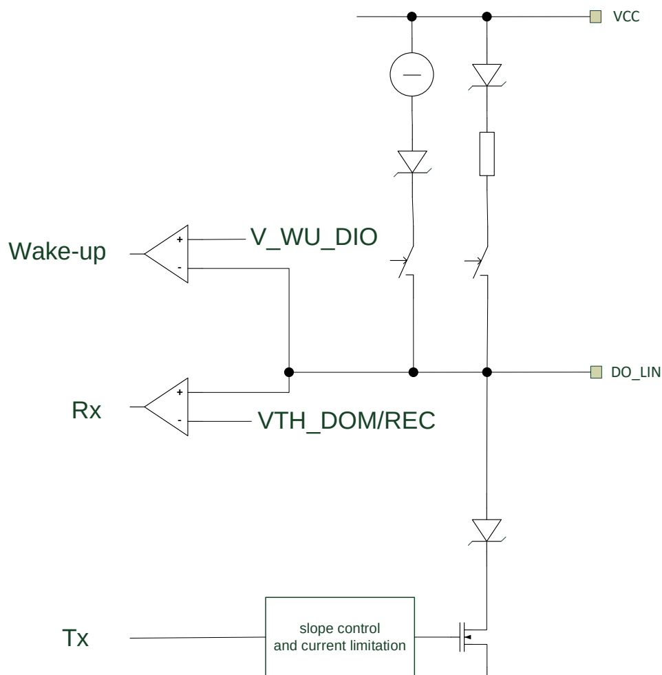
Figure 7. DIO_BUS/DO conceptual schematic
