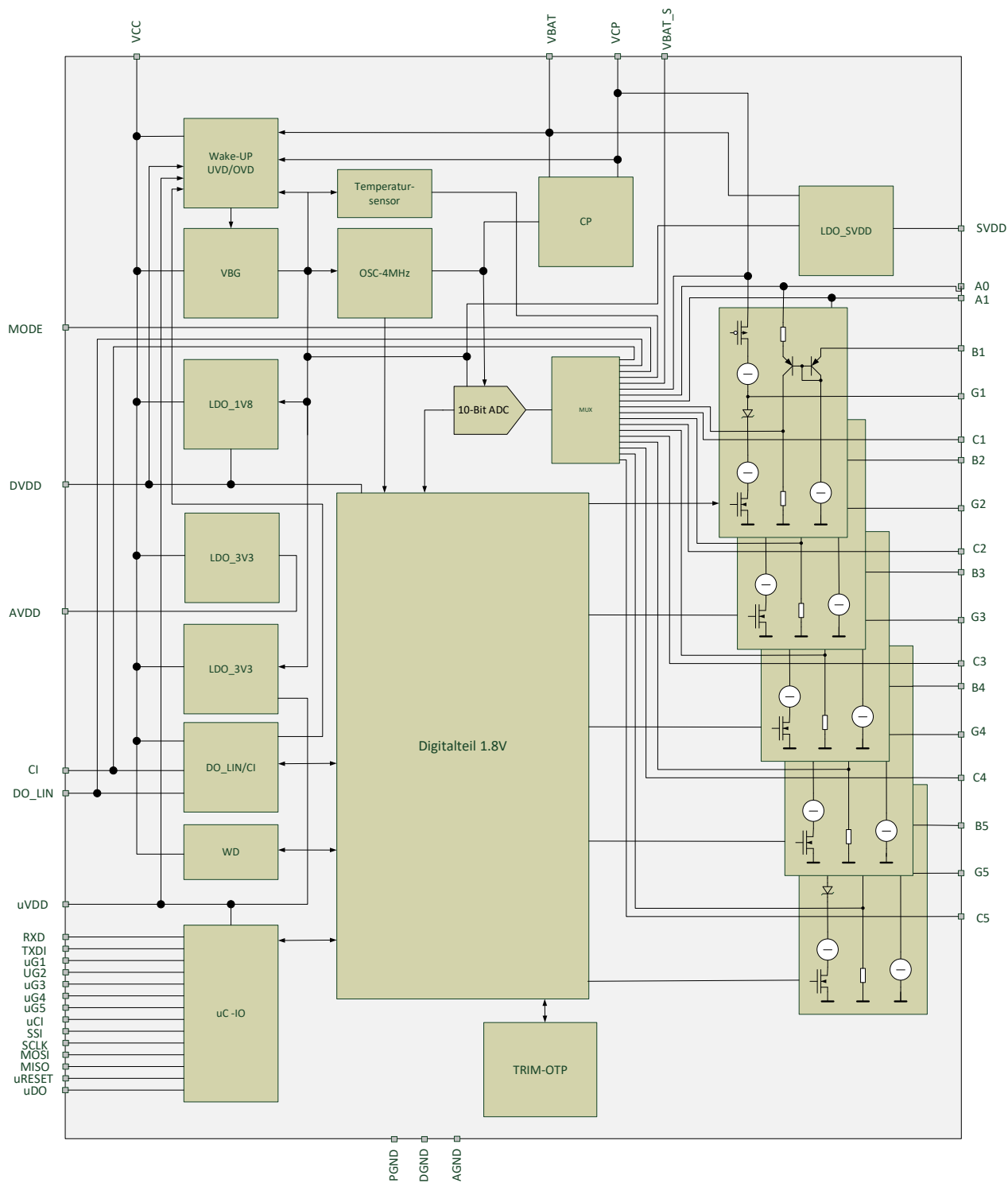
Figure 1. Block diagram
