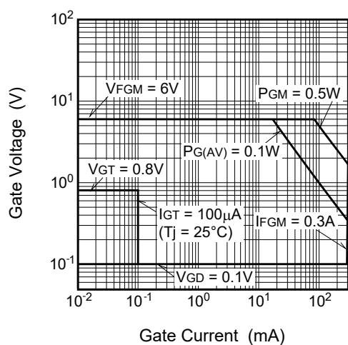
Gate Characteristics
