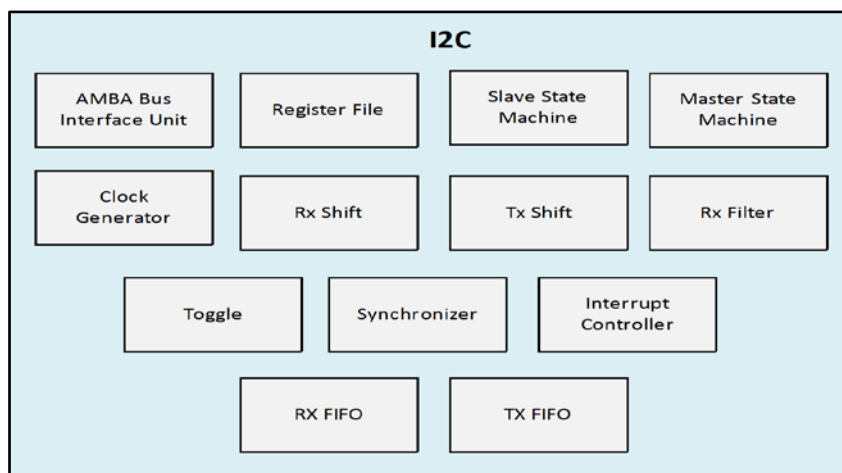
Figure 24: I2C Controller Block Diagram
