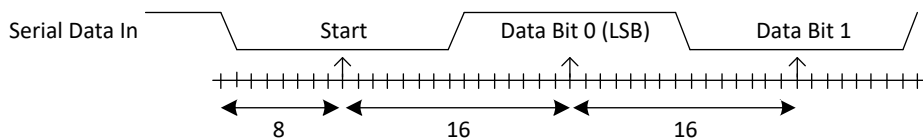
Figure 38. Receiver serial data sampling points
