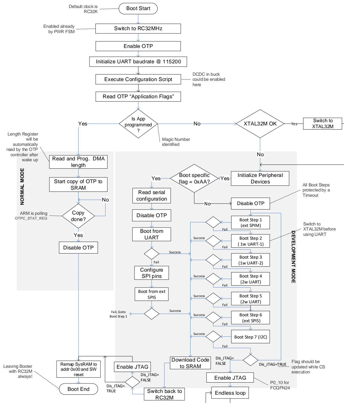
Figure 12. BootROM sequence
