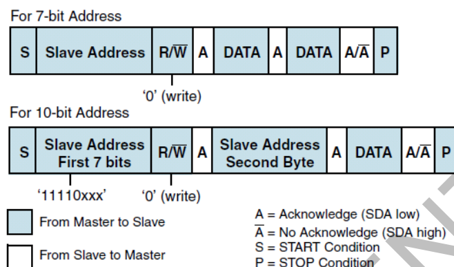
Figure 23: Master-Transmitter Protocol
