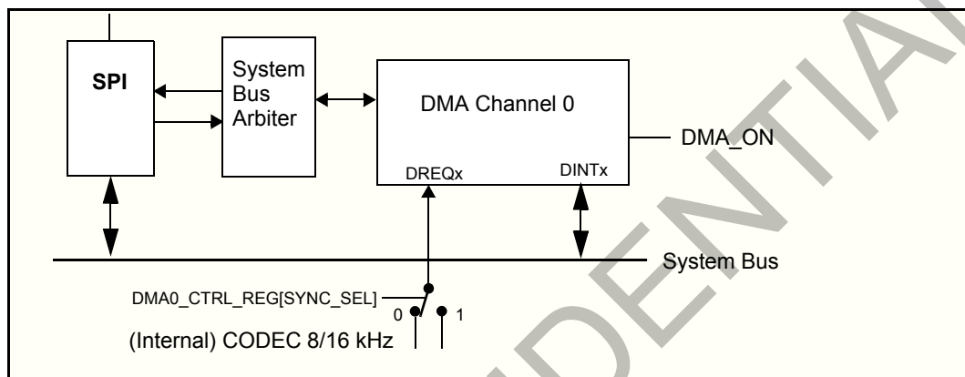
Figure 64: DMA Controller Block Diagram
