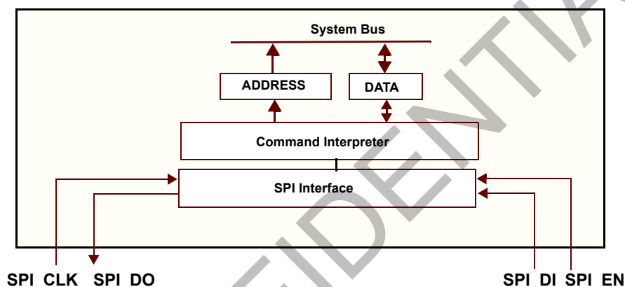
Figure 59: SPI Block Diagram
