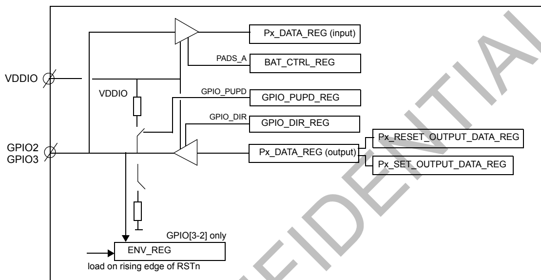
Figure 67: CODEC GPIO Ports
