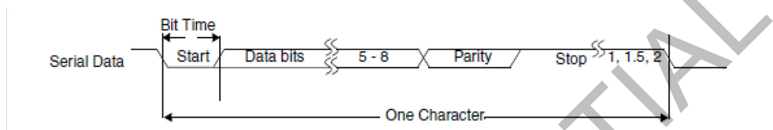
Figure 29: Serial Data Format
