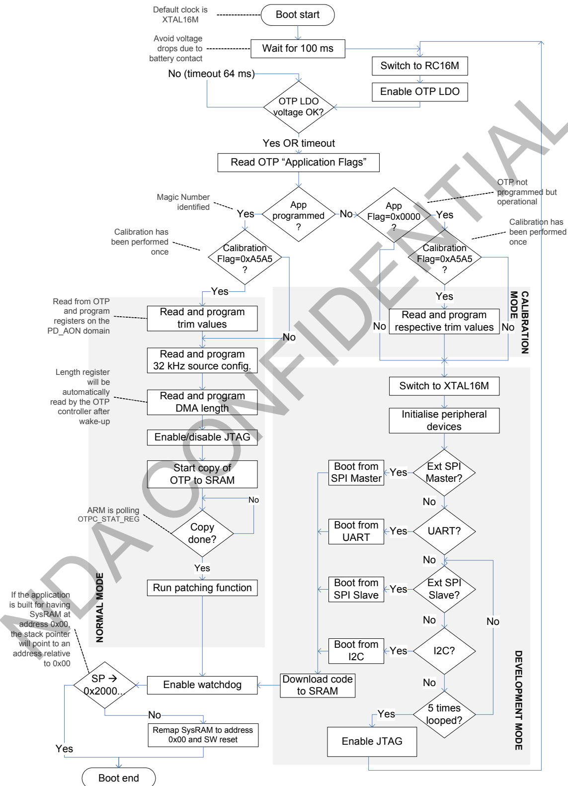
Figure 7: BootROM Sequence
