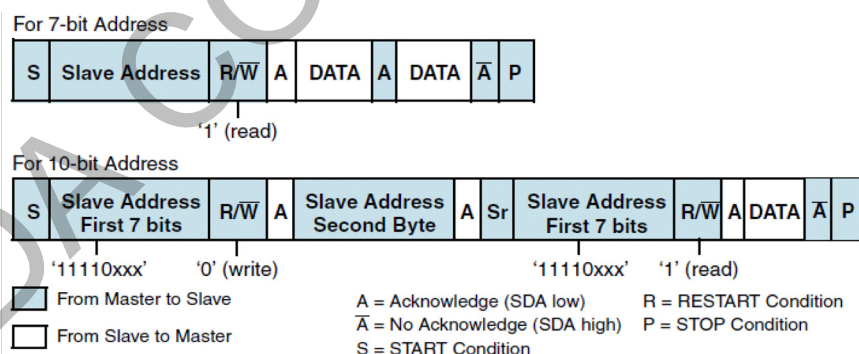
Figure 24: Master-Receiver Protocol
