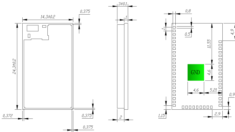
Figure 8. AAC module dimension
