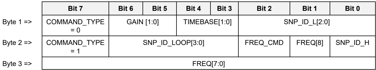
Figure 28. Command structure for a single frame
