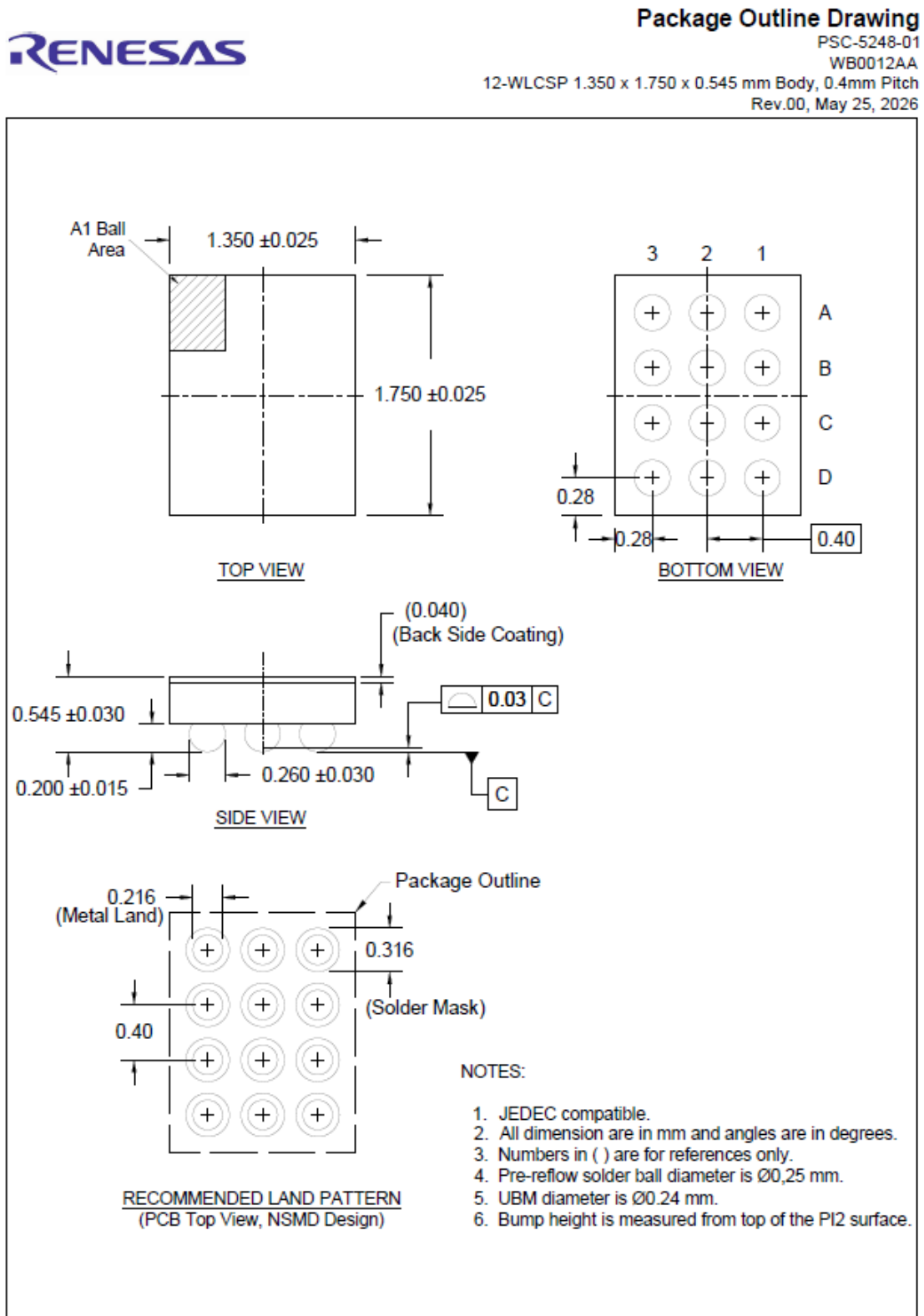
Figure 40. WLCSP package outline drawing
