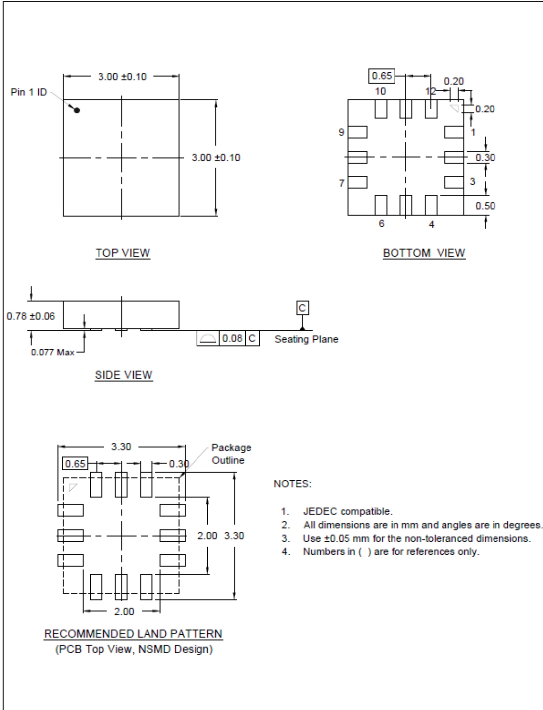
Figure 41. QFN package outline drawing
