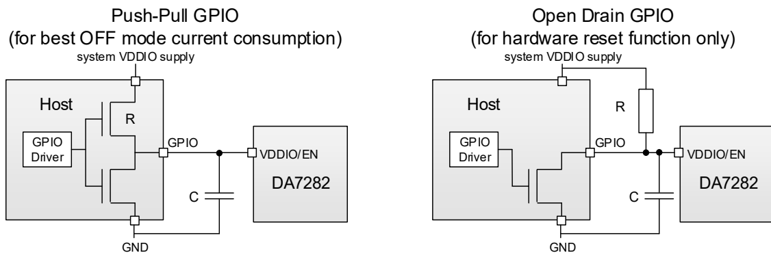
Figure 24. VDDIO pin control in push-pull configuration and open drain configuration
