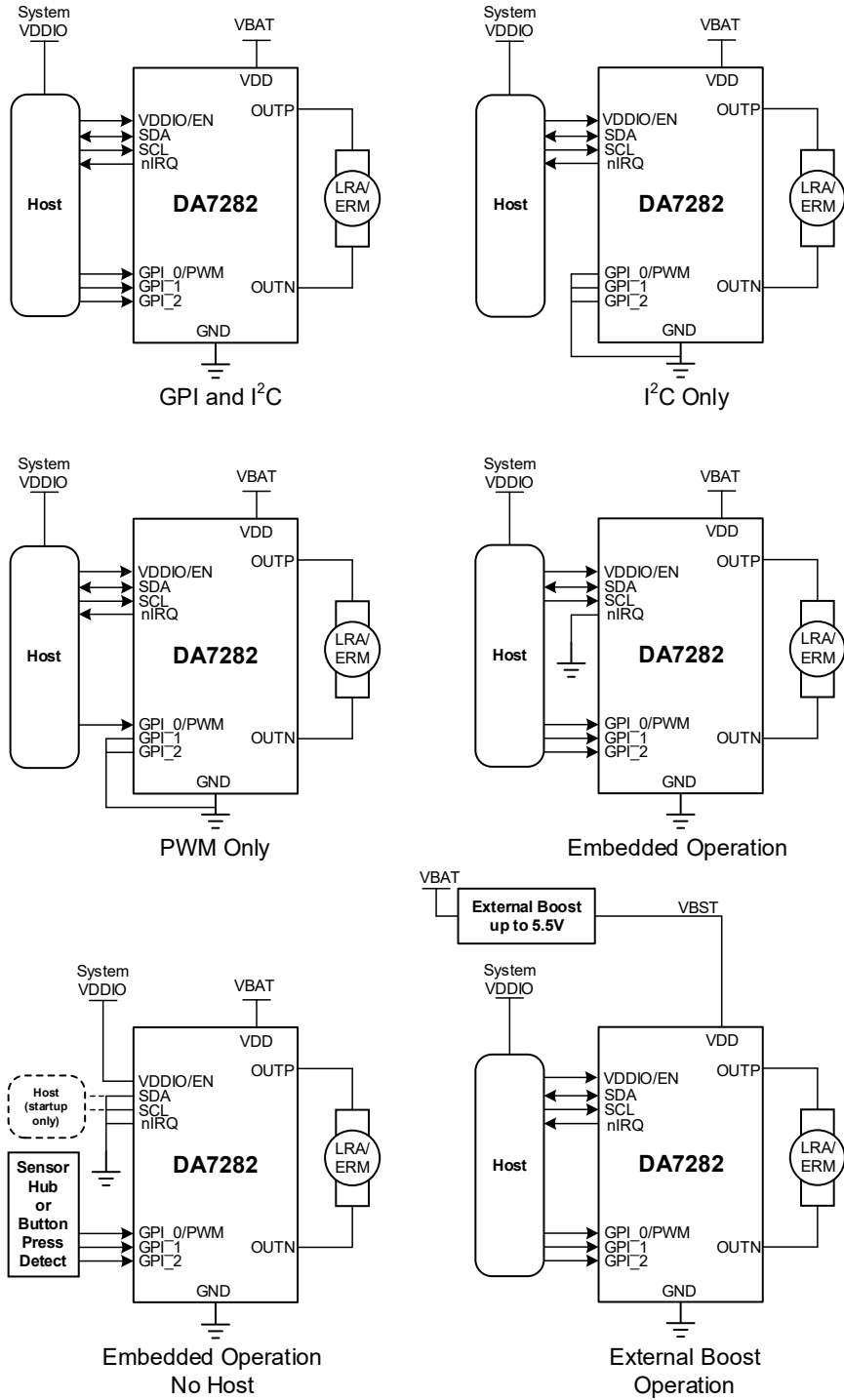
Figure 1. System diagrams
