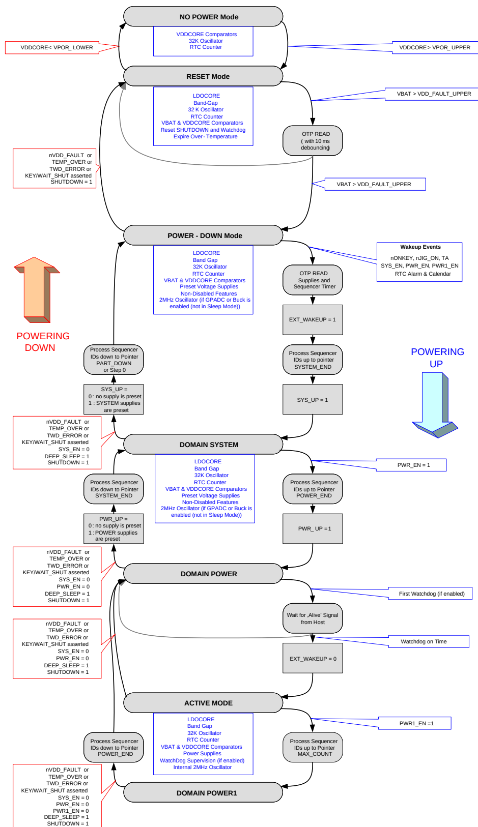
Figure 12: Operating Modes
