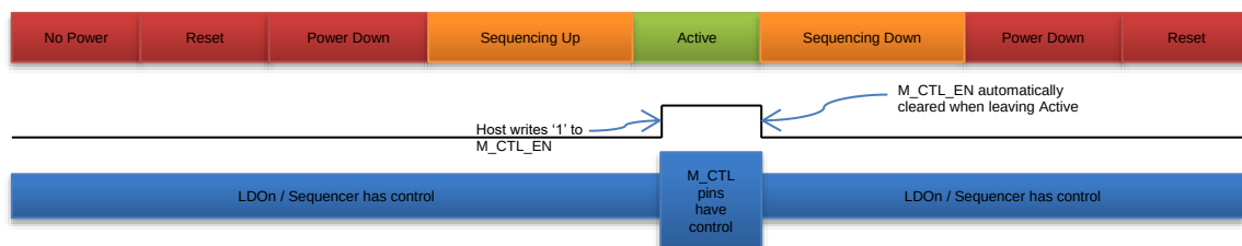
Figure 18: Control from MCTL pins
