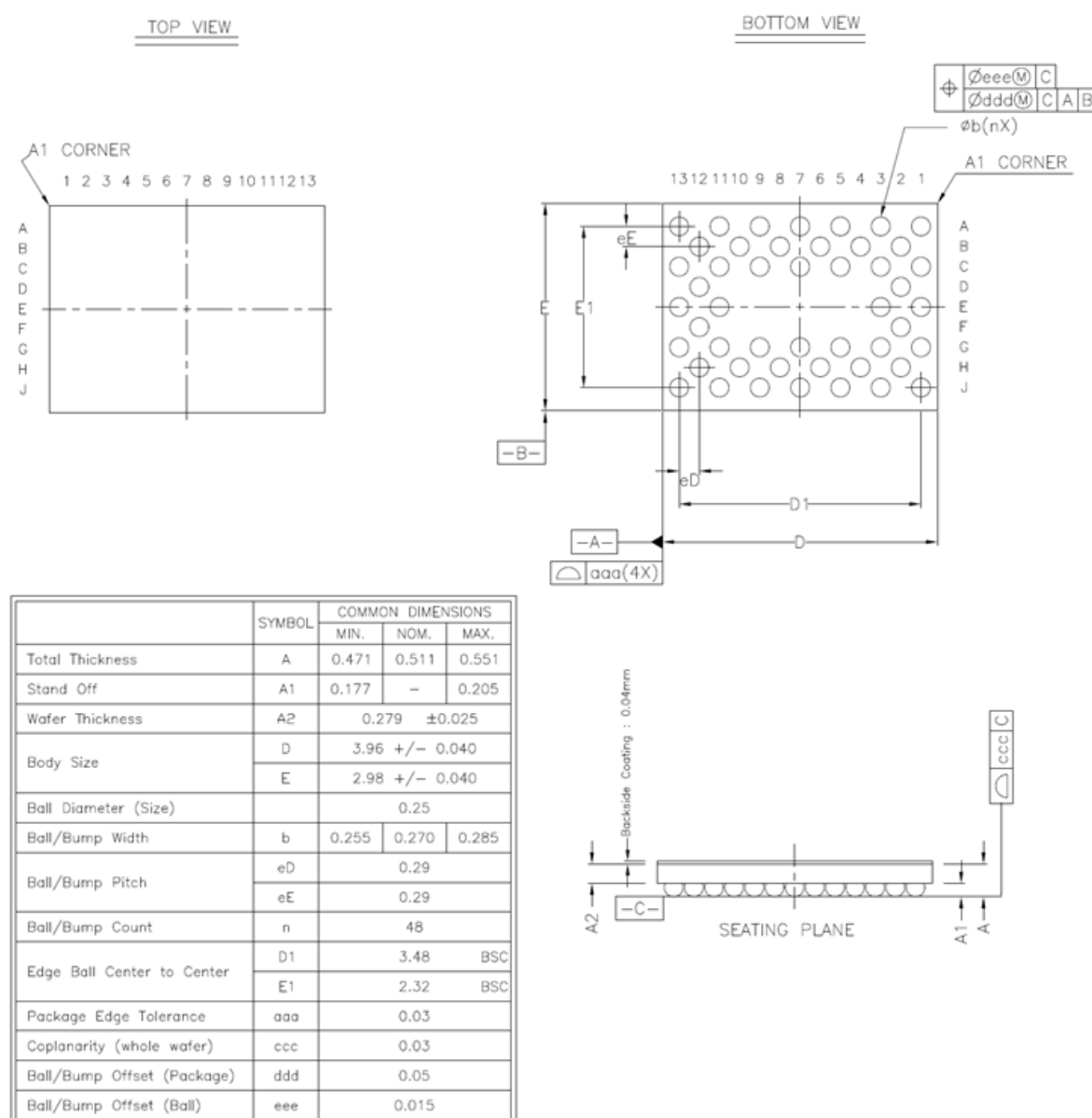
Figure 48: Package Outline Drawing (48 WLCSP)
