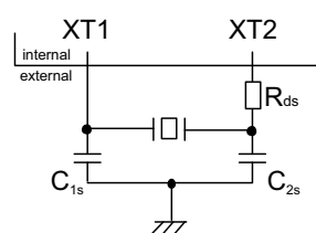
Figure 4-2 Recommended Sub Oscillator Circuit
